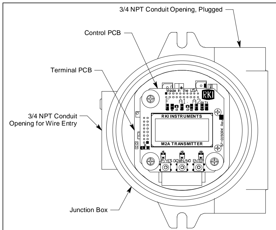
Figure 10: M2A Internal Components
