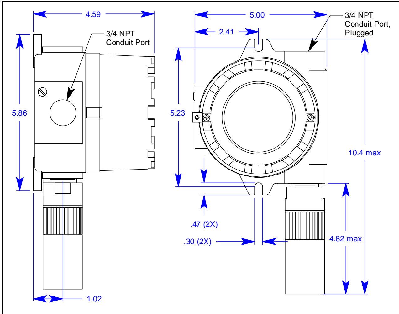
Figure 20: Outline & Mounting Dimensions, ESM-01 Toxic
