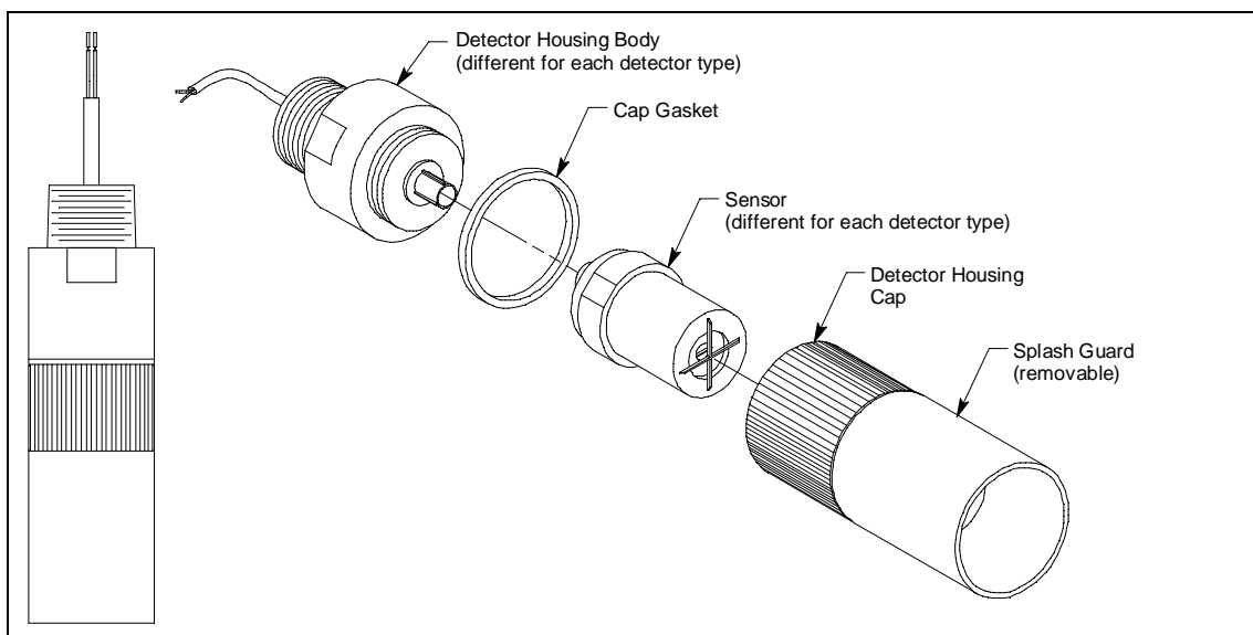
Figure 7: ESM-01 Type Detector
