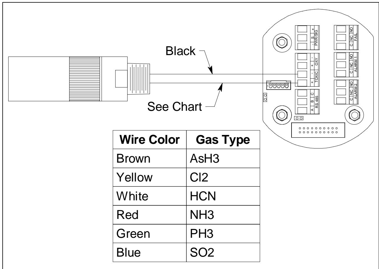
Figure 29: ESM-01 Toxic Detector Wiring
