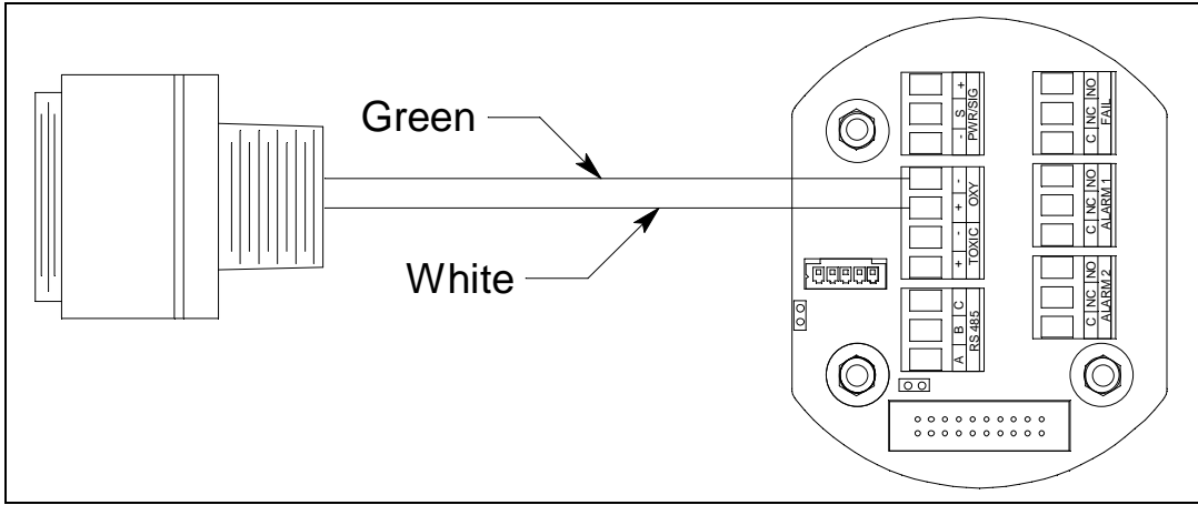
Figure 26: Capillary Type Replaceable Sensor Oxygen Detector Wiring
