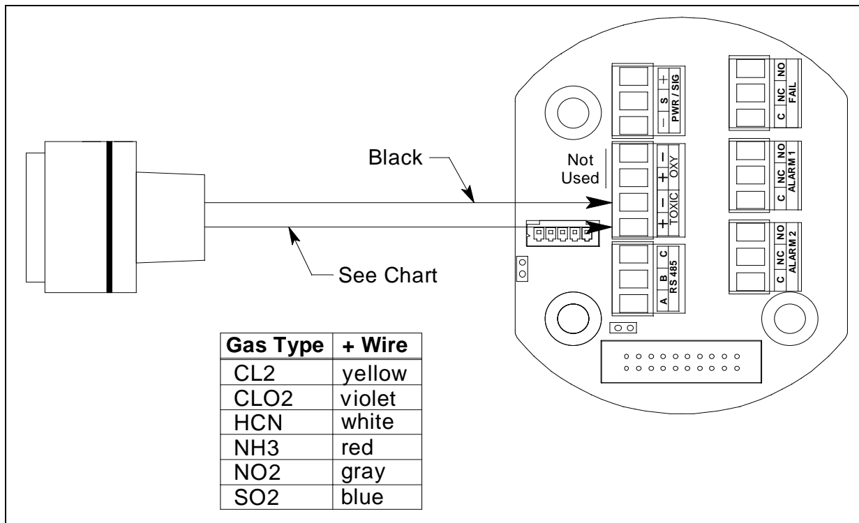
Figure 30: Non-Explosion Proof CT-7 Series Toxic Detector Wiring
