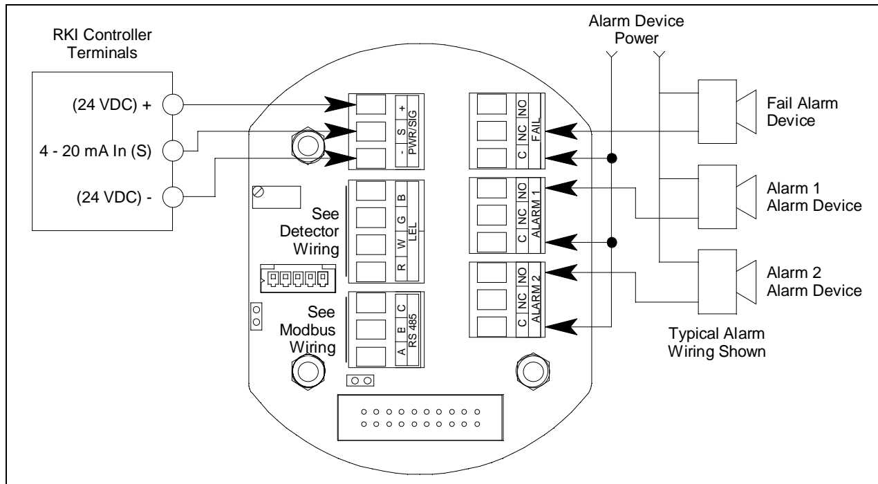
Figure 31: Wiring the M2A to a Controller and Alarm Devices
