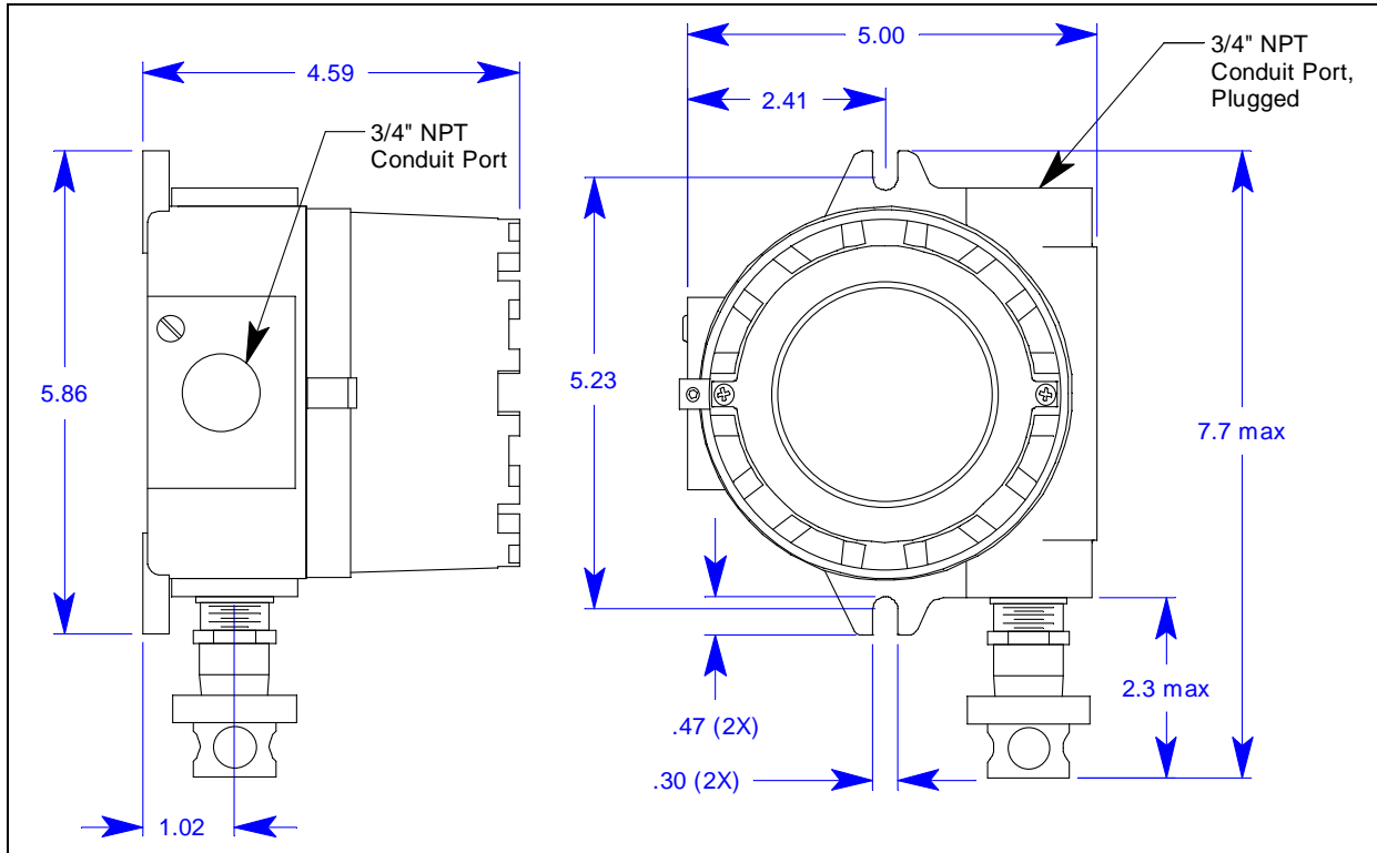
Figure 15: Outline & Mounting Dimensions, Catalytic LEL and ppm, CSA Version
