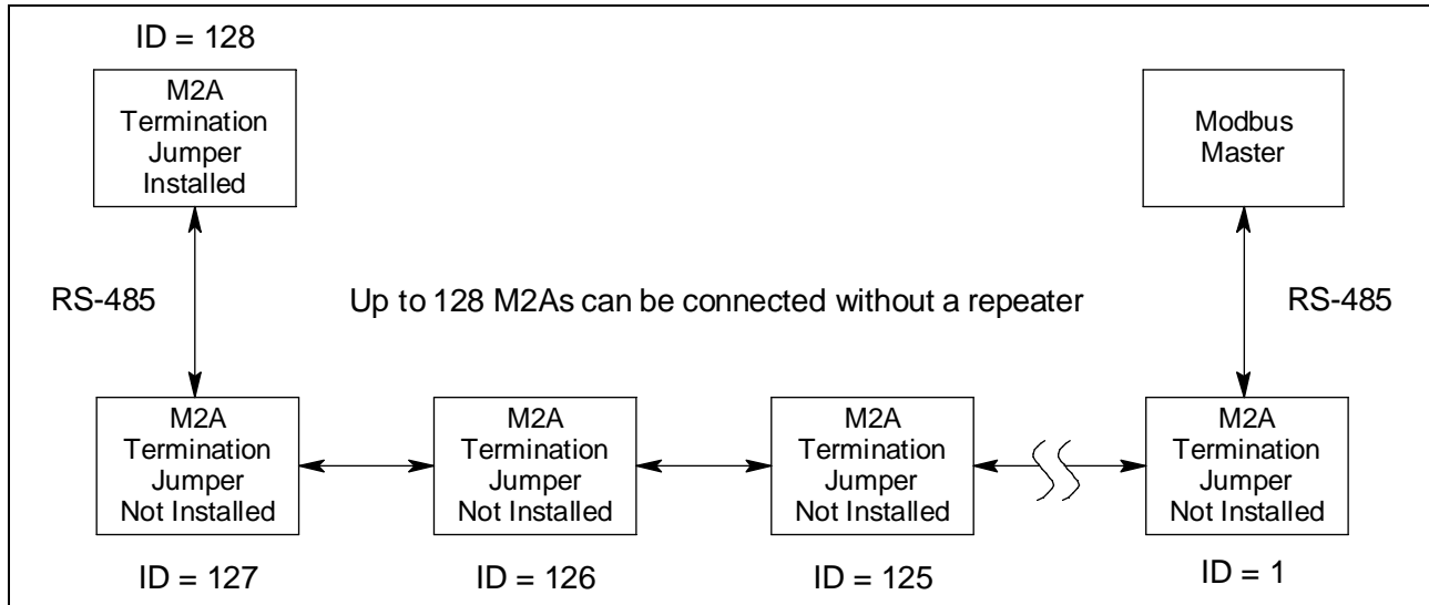
Figure 35: Multiple M2As in a Daisy Chain Configuration
