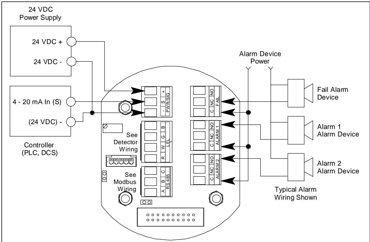
Figure 37: PLC and DCS Device Wiring
