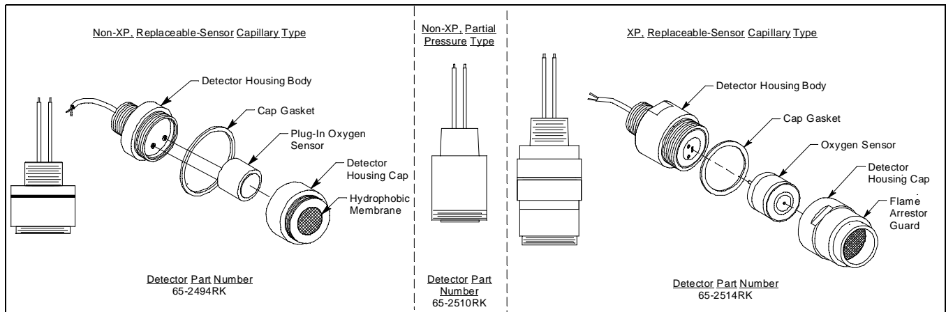
Figure 4: Oxygen Detectors
