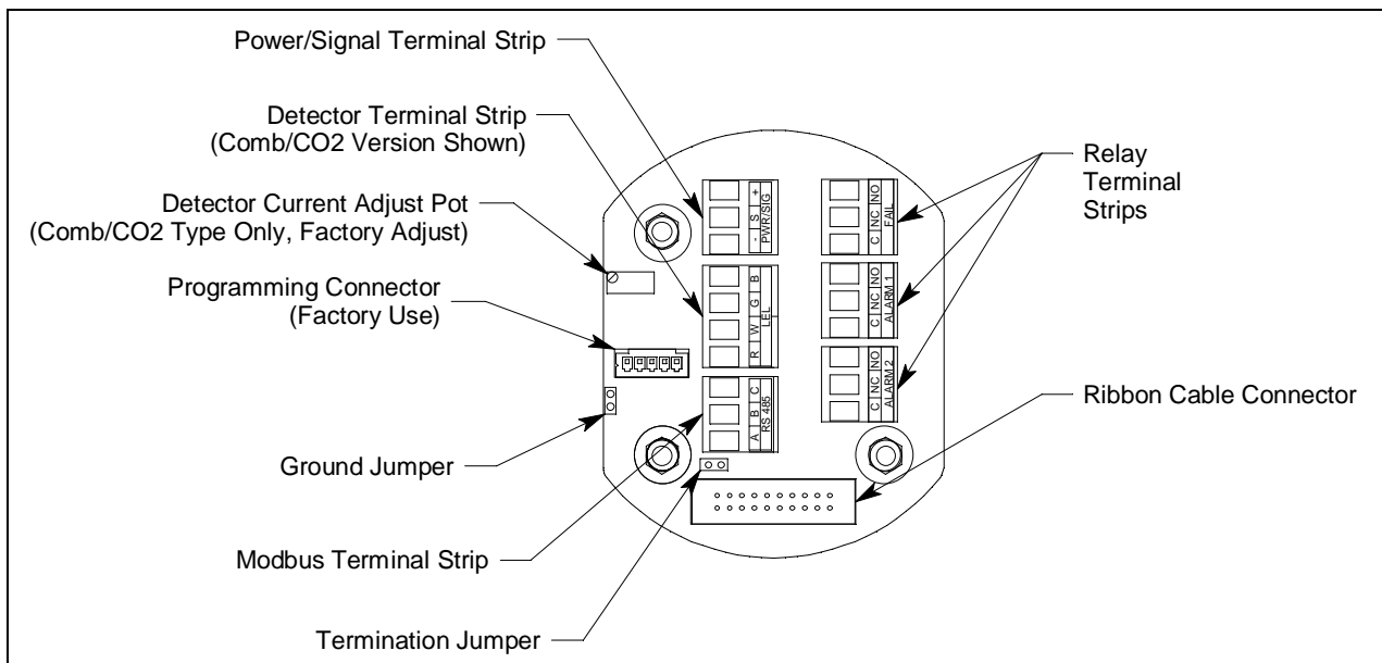
Figure 11: Terminal PCB Component Location
