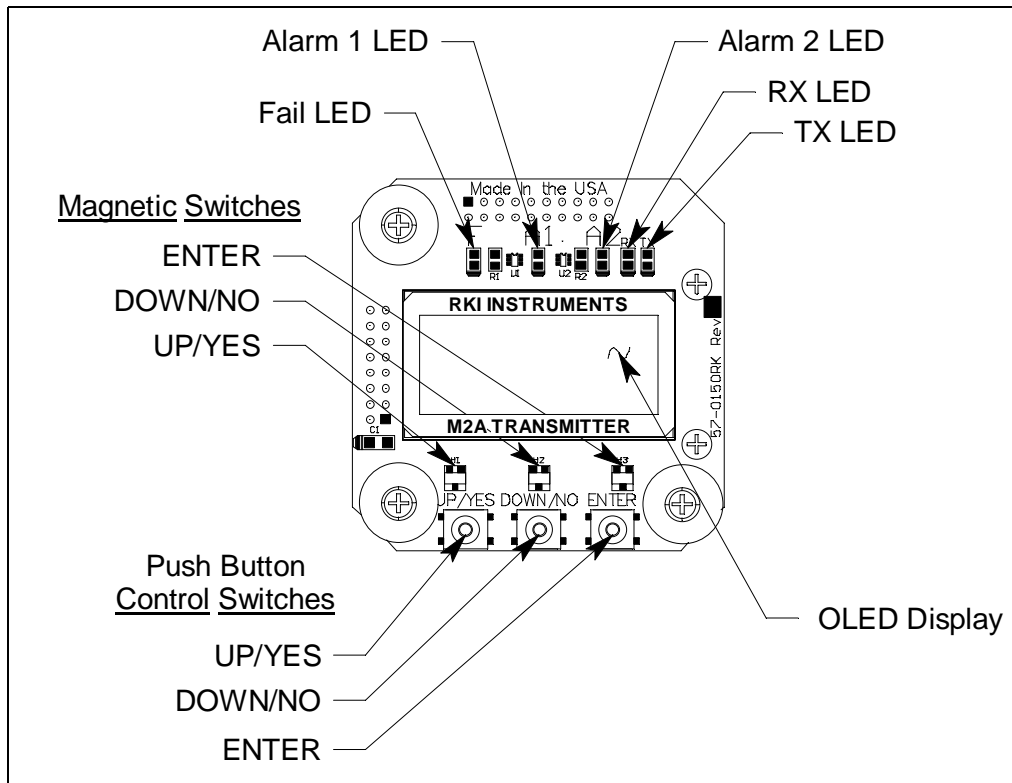
Figure 13: Control PCB Component Location
