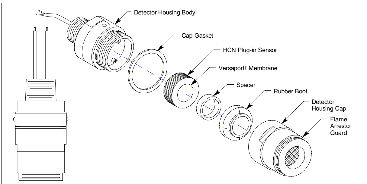
Figure 9: Explosion-Proof CT-7 Series HCN Detector
